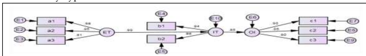
Figure (3): Path of the Full Model Using SEM
